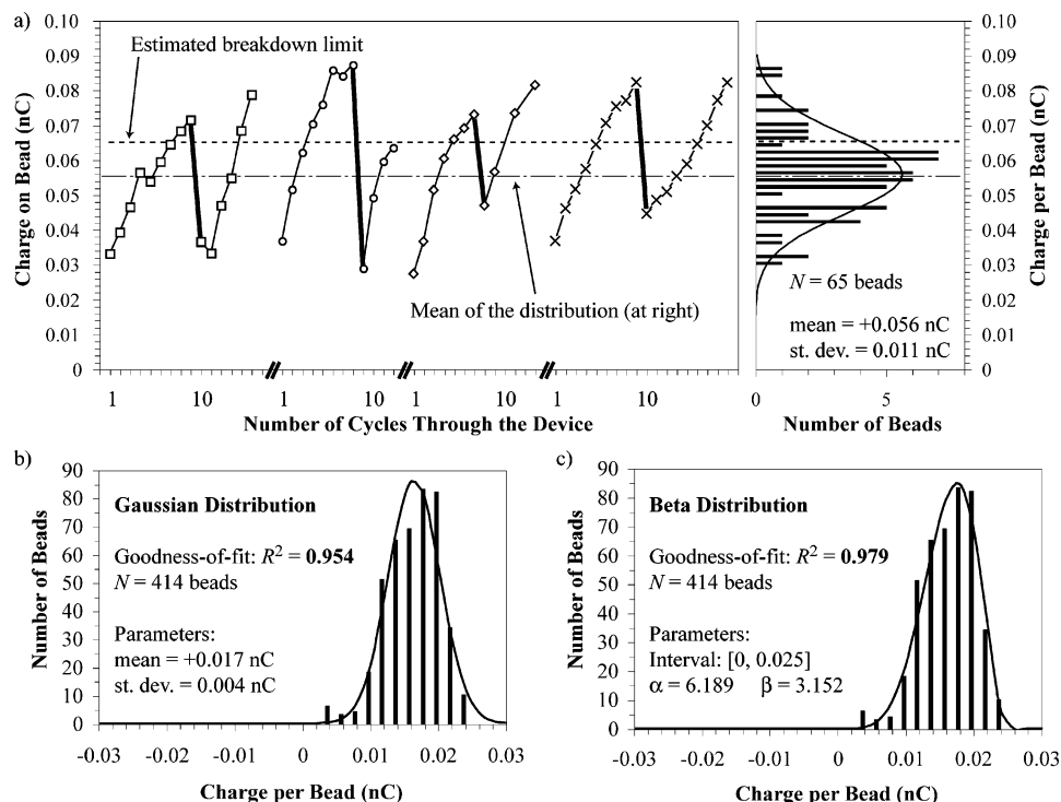
Figure 8. (a) The left graph shows repeated measurements of charge on four different 450- \mu\text{m} -diameter microspheres with tetraalkylammonium functionality (1); the right graph shows a histogram of single measurements of charge for 65 such beads. (b) Histogram of the measurements of charge of 200- \mu\text{m} -diameter microspheres with tetraalkylammonium functionality (1), fit with a Gaussian distribution. (c) The same histogram shown in panel b, fit with a \beta -distribution.
