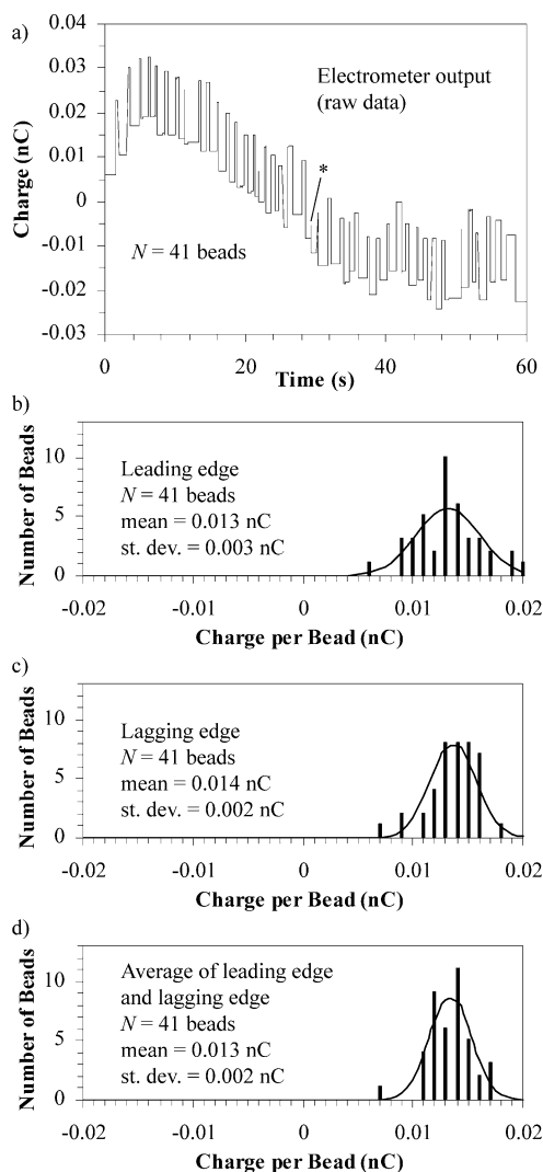
Figure 4. (a) The electrometer output from the measurement of 41 positively charged 200- \mu\text{m} -diameter beads with alkytriphenylphosphonium functionality ( 3 ); contact with aluminum charged the beads. The peak indicated with an asterisk (*) was excluded from the data analysis for reasons explained in the text. (b-d) Histograms of the measurements of charge extracted from the electrometer output shown above; the superimposed curve is the normal distribution calculated from the mean and standard deviation: (b) the leading-edge charge, (c) the lagging edge charge, and (d) the average of the leading-edge and lagging-edge charge.
